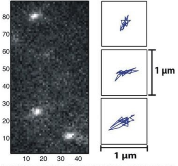
Figure 2. An SMLM image of single molecule EGFs in a living cell taken with an exposure time of 20 ns. Three typical trajectories of EGFs observed in confined regions were extracted from sequential exposures using the software mentioned in the text.
